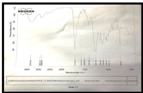
Fig (3): Graft co-polymer's FT-IR spectra
