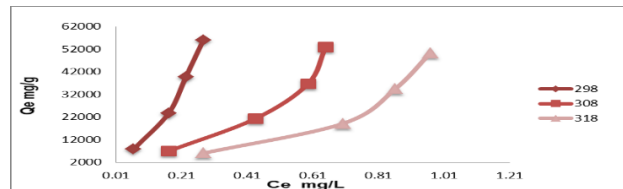
Fig11. Shows the effect of temperature on the polymer at concentrations (1, 3, 5 and 7 ppm) and temperatures (298, 308 and 318)
