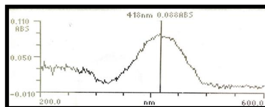
Fig (9) maximum wavelength (λ max) for the (Reactive Yellow 145)
